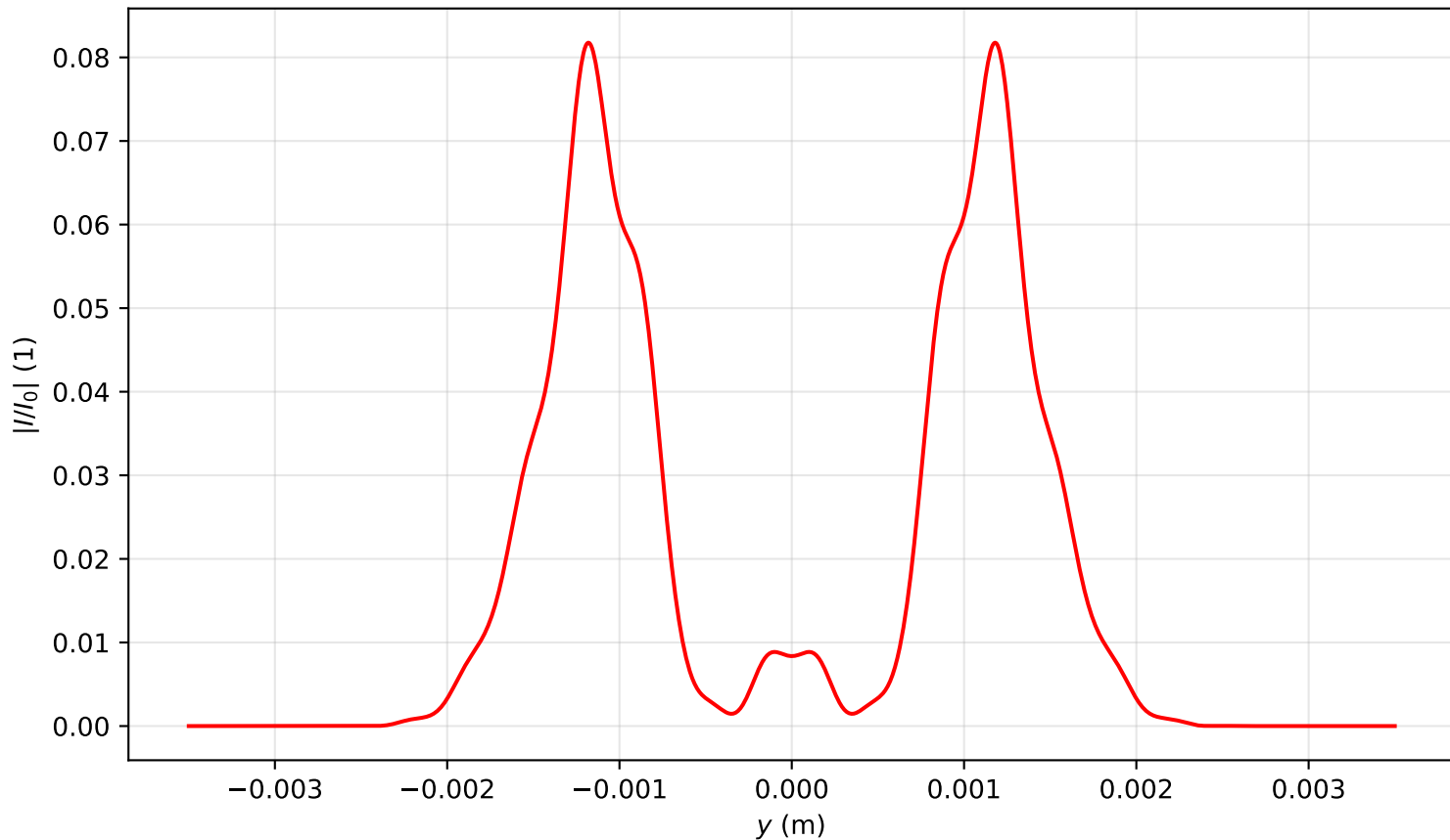
Intensity profile I(x=0, y, z=3.344)/I_0 , P_{in}=7.0P_{cr} , artificial time
